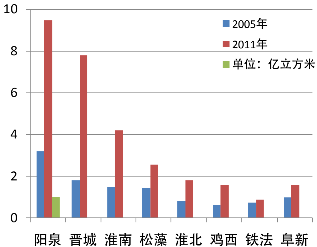
Comparison of CMM Drainage Volume in 2005 and 2011 of 8 Key State Owned Coal Mining Groups
